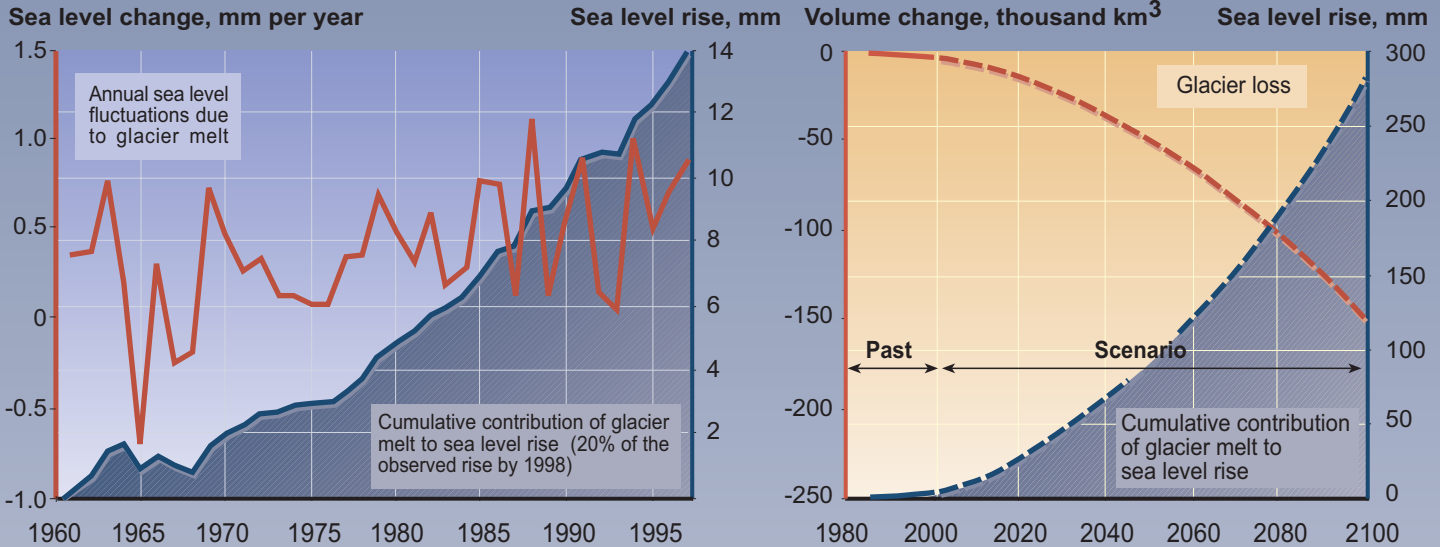
Global average sea level rise, mm
