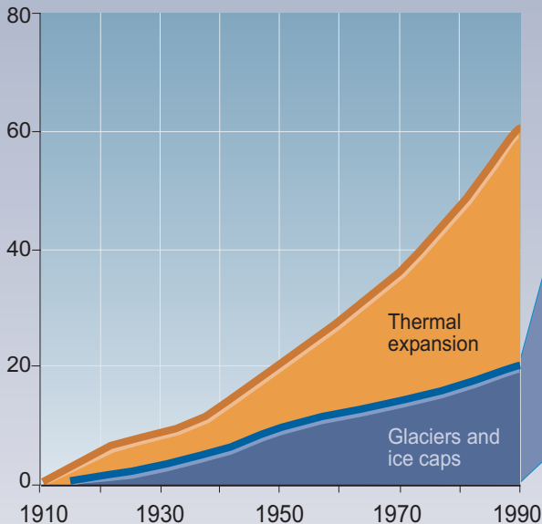
Global average sea level rise, mm
