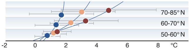
d) E Greenland, Scandinavia, NW Russia
