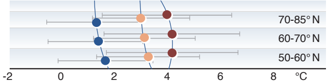
b) Chukotka, Alaska, western Canadian Arctic
