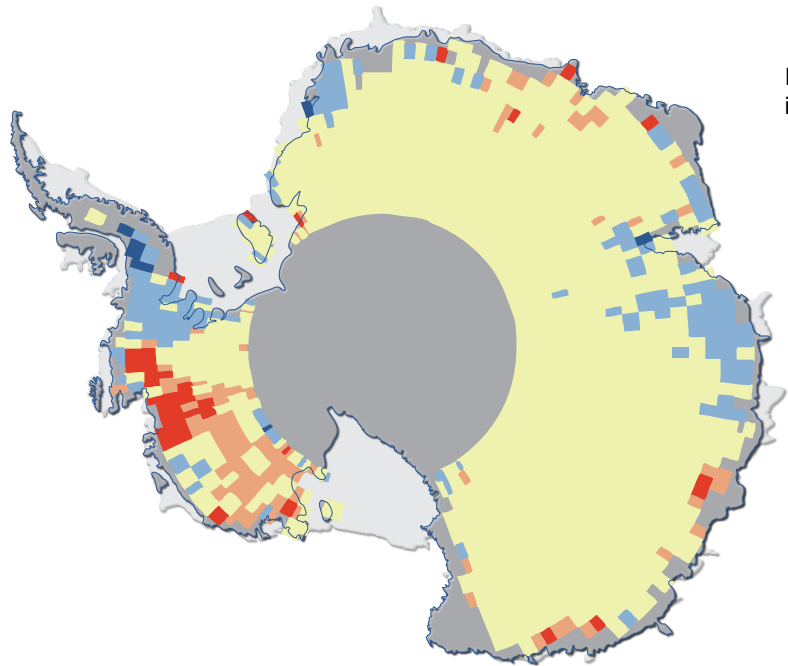
Surface-elevation change (cm/year)
