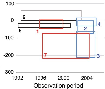
Rate of mass increase (billion tonnes/year)
