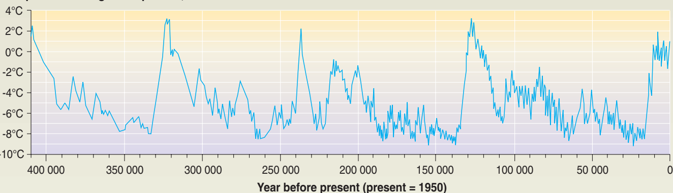
Temperature change from present, °C
