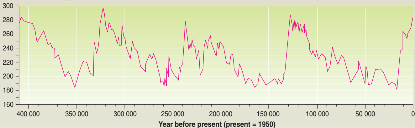
CO 2 concentration, ppmv
